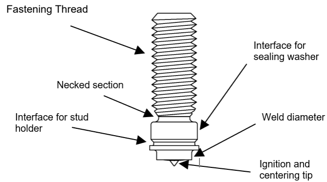
FIGURE 1—F-BT STUD TERMINOLOGY
